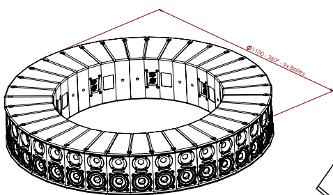
Example of 360° configuration (Dimensions in mm)
